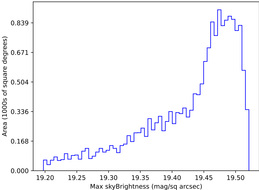
noroll_v3.4_10yrs WFD z band: Max skyBrightness
