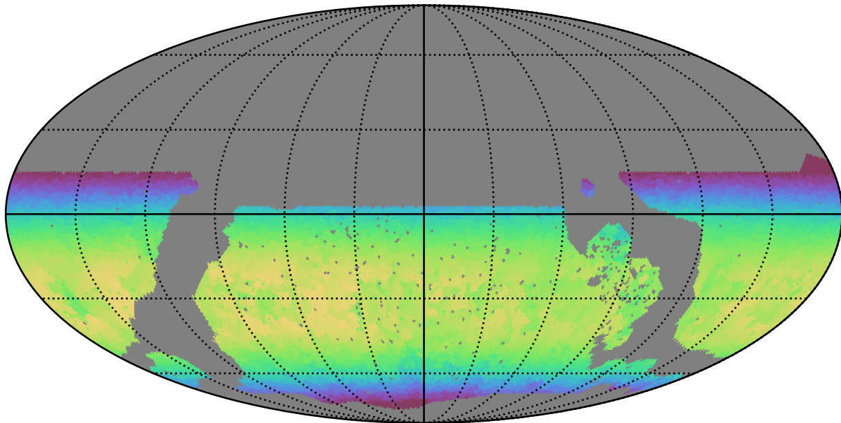
noroll_v3.4_10yrs WFD y band: Max skyBrightness
