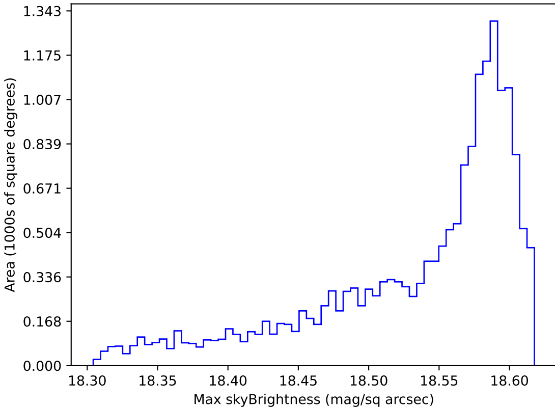
noroll_v3.4_10yrs WFD y band: Max skyBrightness
