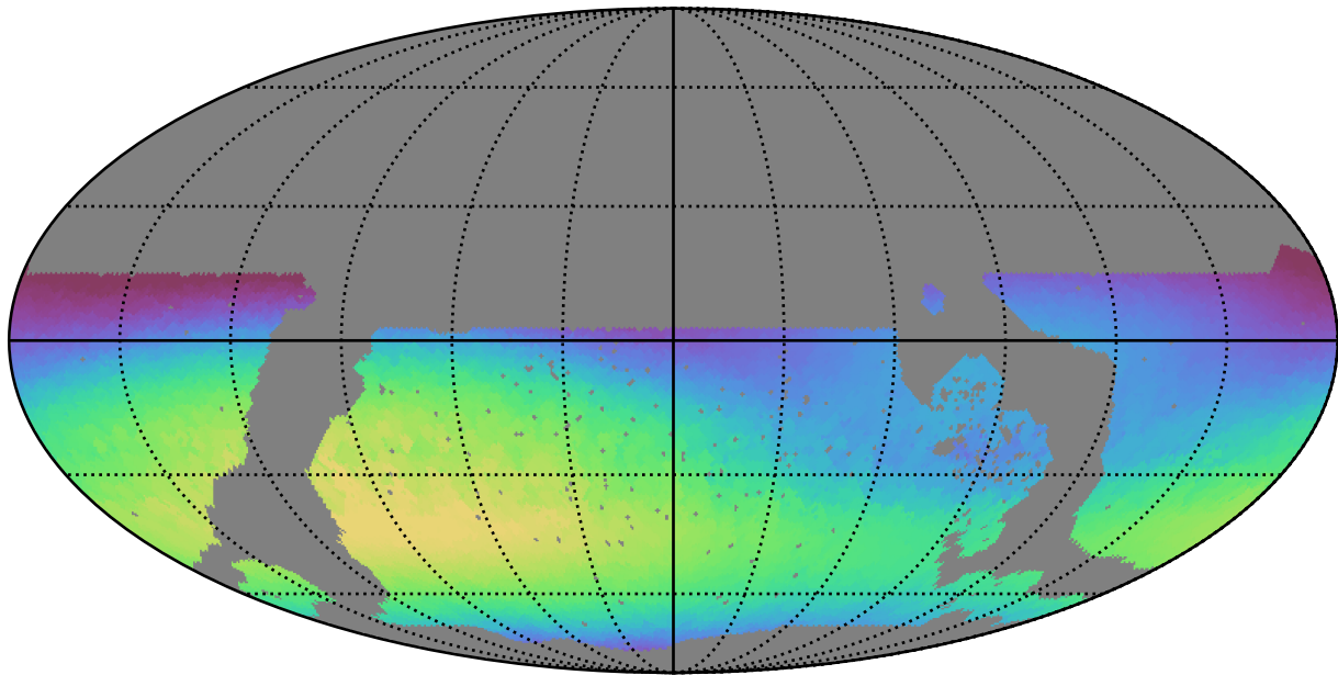
noroll_v3.4_10yrs WFD u band: Max skyBrightness
