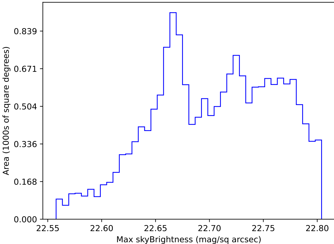
noroll_v3.4_10yrs WFD u band: Max skyBrightness
