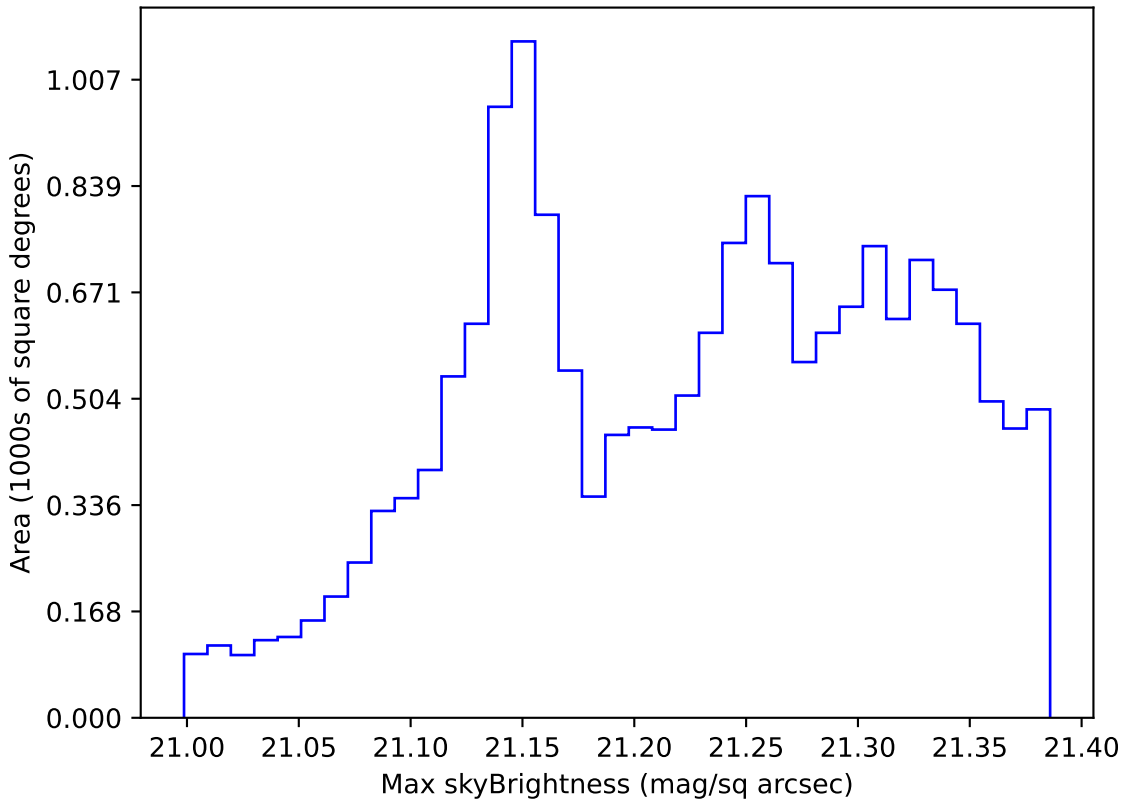
noroll_v3.4_10yrs WFD r band: Max skyBrightness
