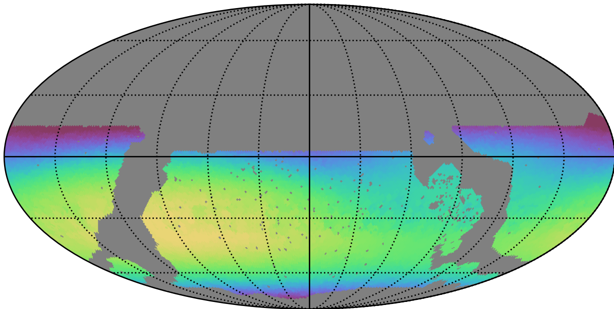
noroll_v3.4_10yrs WFD i band: Max skyBrightness
