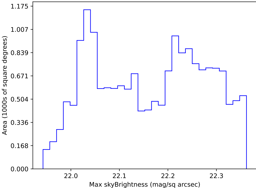
noroll_v3.4_10yrs WFD g band: Max skyBrightness
