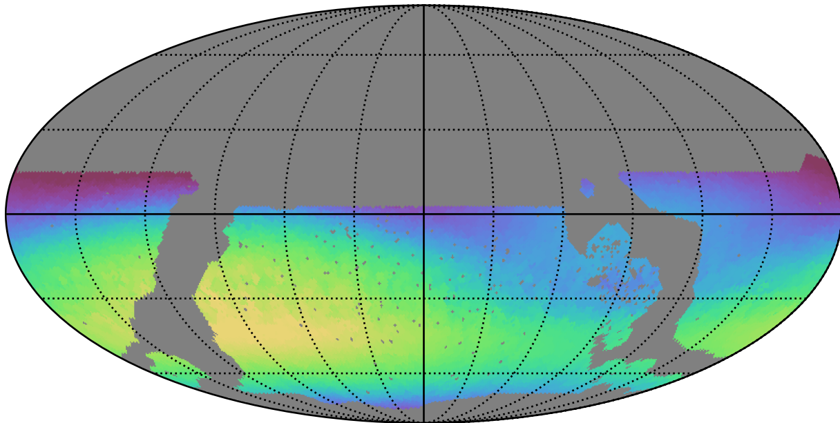
noroll_v3.4_10yrs WFD all bands: Max skyBrightness
