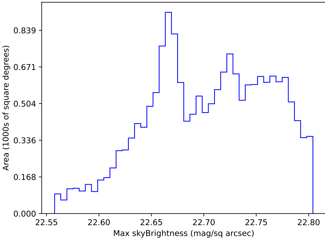
noroll_v3.4_10yrs WFD all bands: Max skyBrightness
