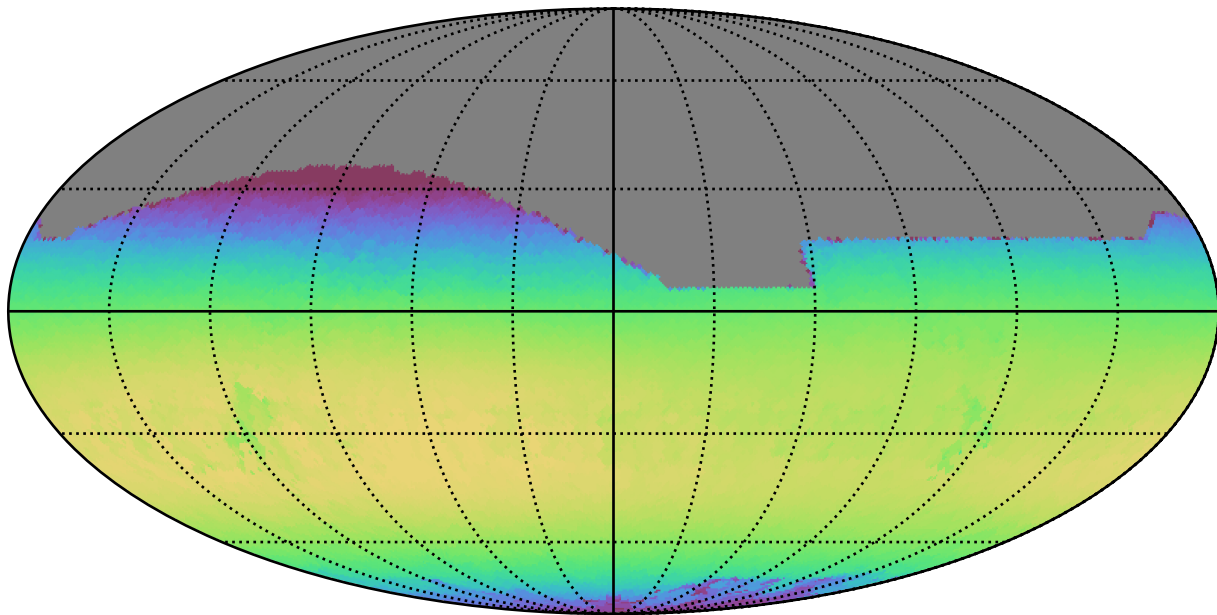
noroll_v3.4_10yrs All sky z band: Max skyBrightness
