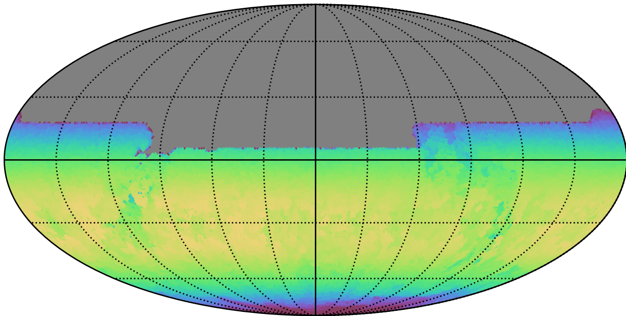
noroll_v3.4_10yrs All sky y band: Max skyBrightness
