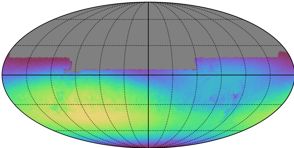
noroll_v3.4_10yrs All sky u band: Max skyBrightness
