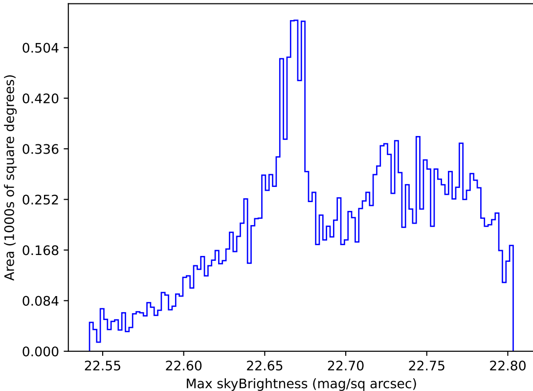
noroll_v3.4_10yrs All sky u band: Max skyBrightness
