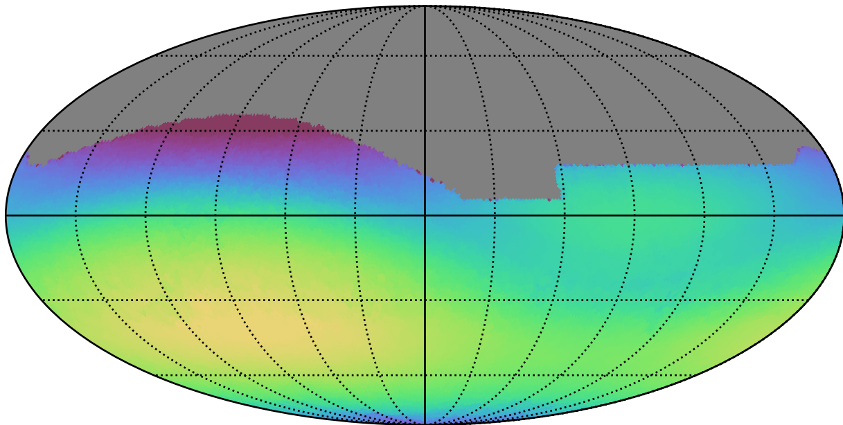
noroll_v3.4_10yrs All sky r band: Max skyBrightness
