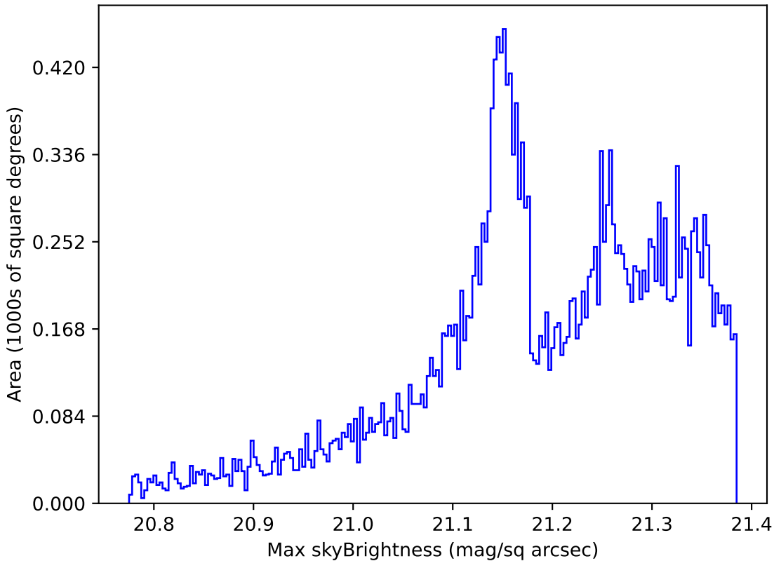
noroll_v3.4_10yrs All sky r band: Max skyBrightness
