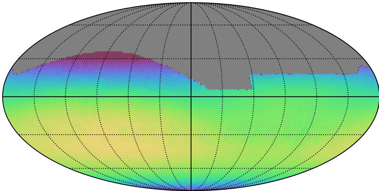
noroll_v3.4_10yrs All sky i band: Max skyBrightness
