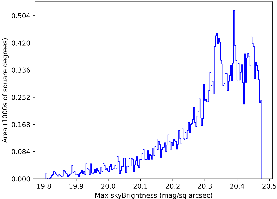
noroll_v3.4_10yrs All sky i band: Max skyBrightness
