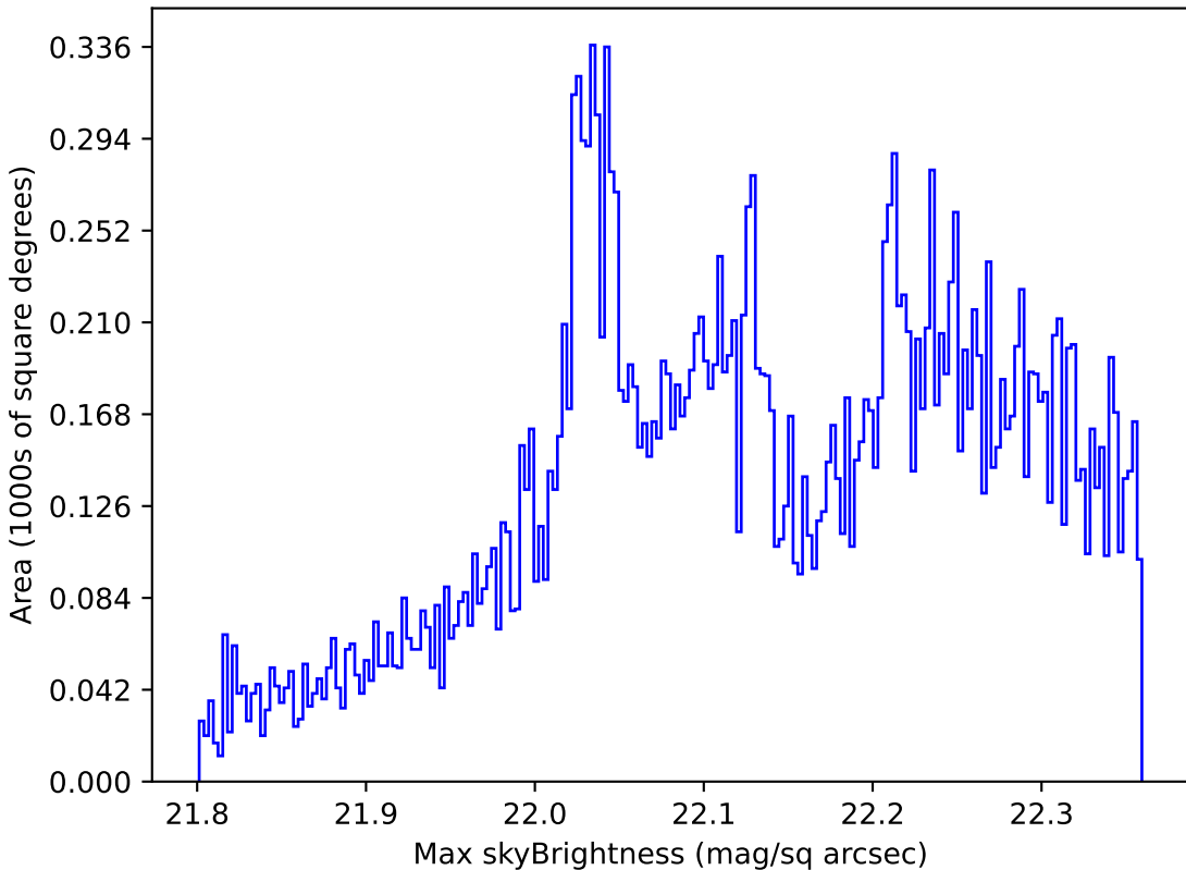
noroll_v3.4_10yrs All sky g band: Max skyBrightness
