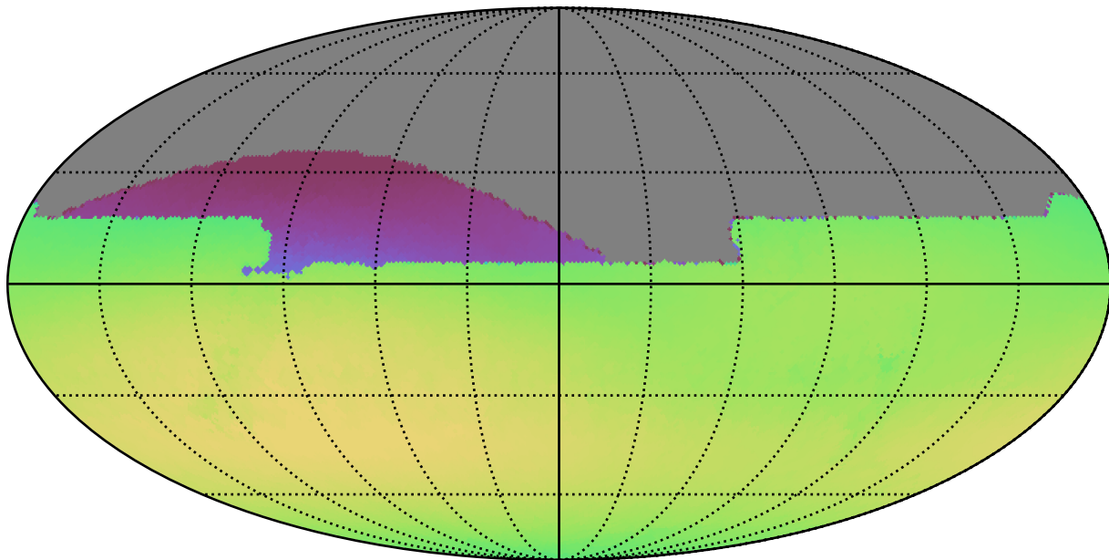
noroll_v3.4_10yrs All sky all bands: Max skyBrightness
