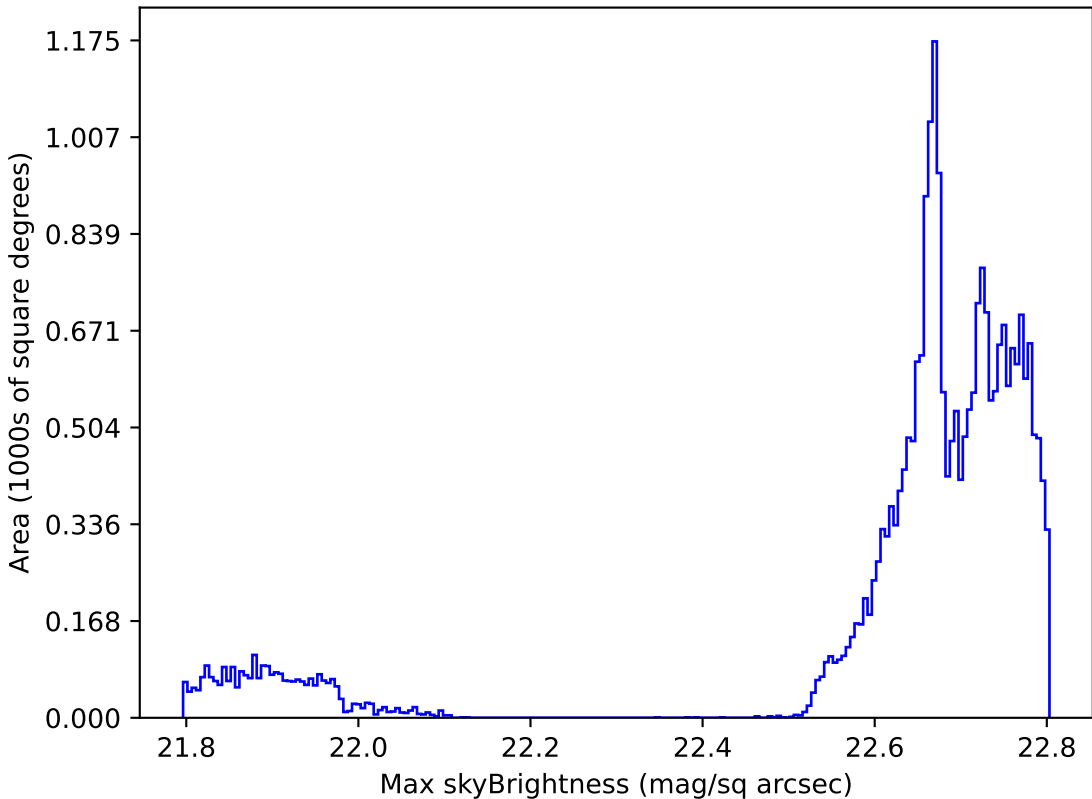
noroll_v3.4_10yrs All sky all bands: Max skyBrightness
