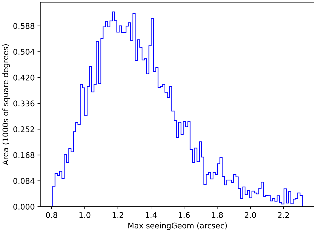
noroll_v3.4_10yrs Yr 1 z band: Max seeingGeom
