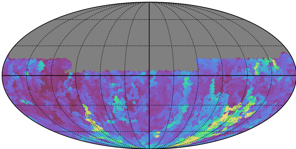
noroll_v3.4_10yrs Yr 1 u band: Max seeingGeom
