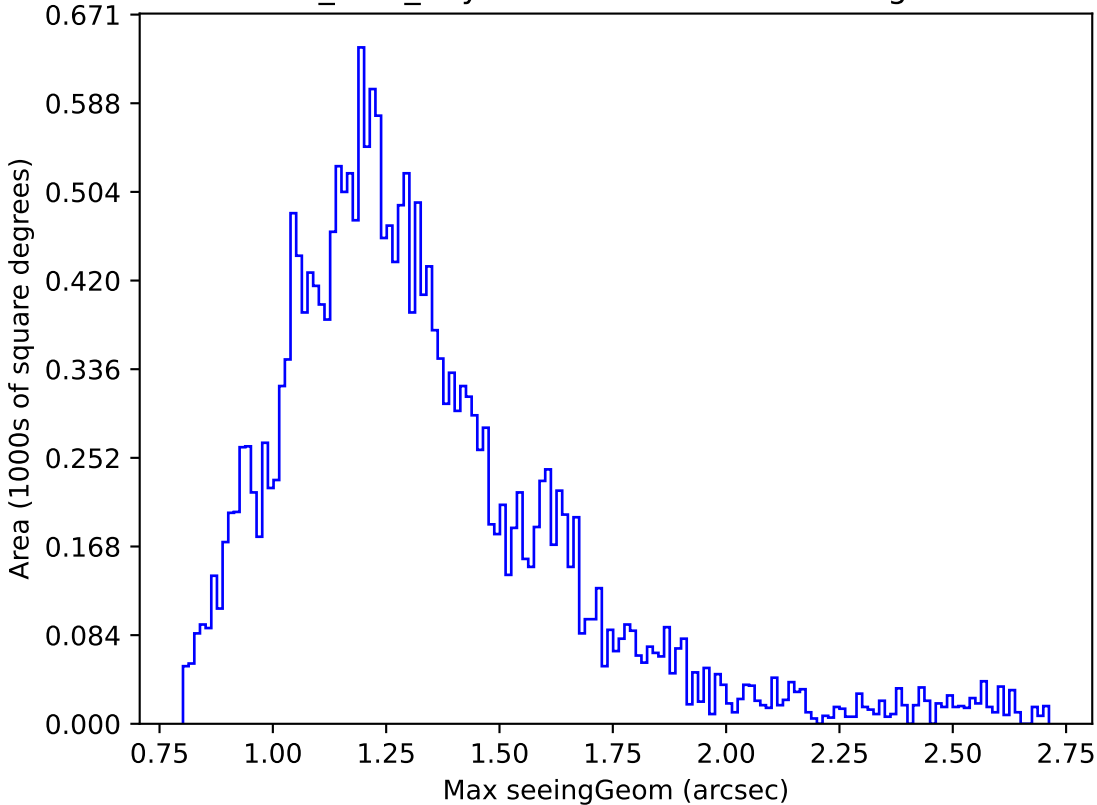
noroll_v3.4_10yrs Yr 1 u band: Max seeingGeom
