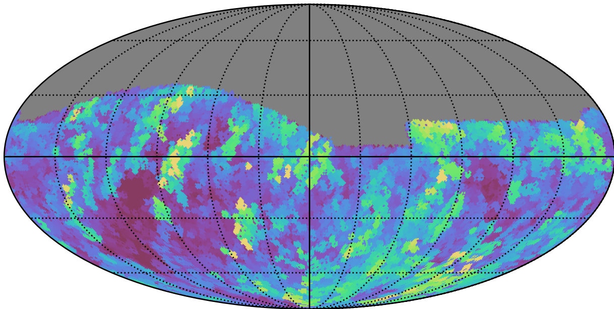
noroll_v3.4_10yrs Yr 1 r band: Max seeingGeom
