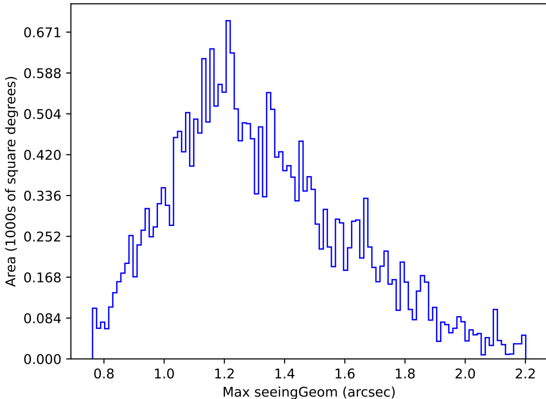
noroll_v3.4_10yrs Yr 1 r band: Max seeingGeom
