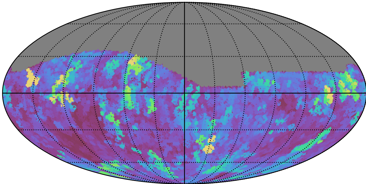
noroll_v3.4_10yrs Yr 1 i band: Max seeingGeom
