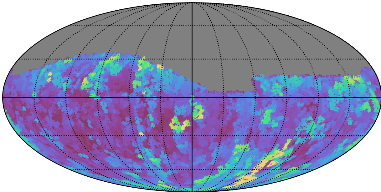
noroll_v3.4_10yrs Yr 1 g band: Max seeingGeom
