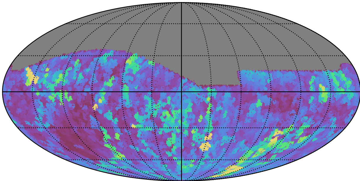
noroll_v3.4_10yrs Yr 1 all bands: Max seeingGeom
