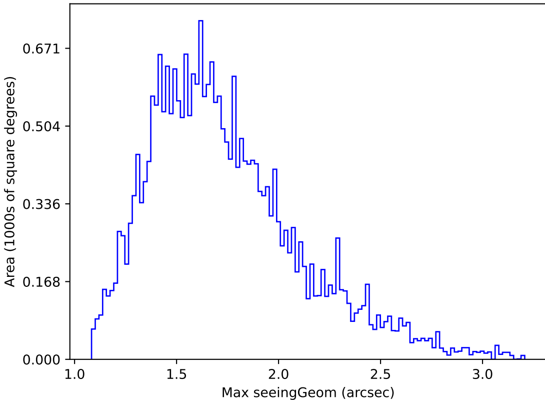
noroll_v3.4_10yrs Yr 1 all bands: Max seeingGeom
