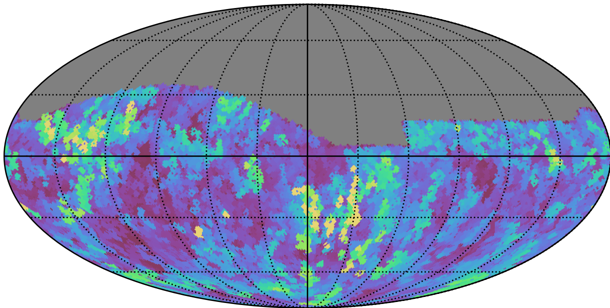
noroll_v3.4_10yrs Yr 1 z band: Max seeingEff
