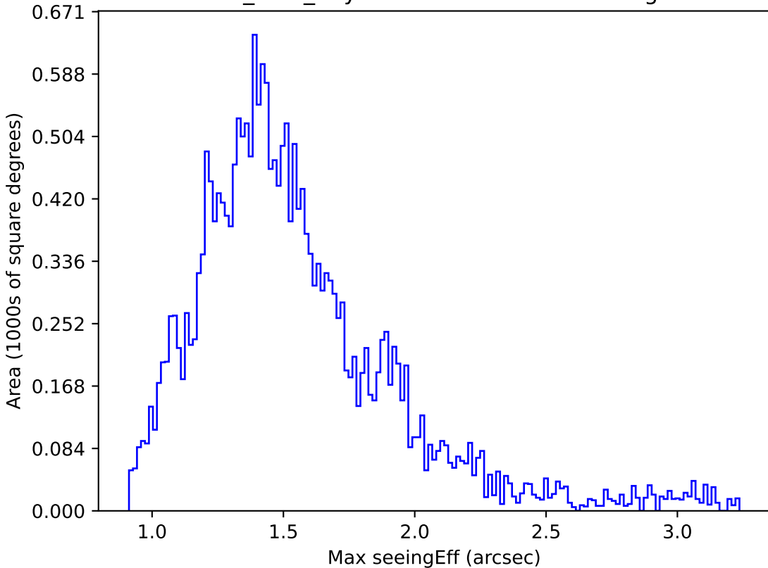
noroll_v3.4_10yrs Yr 1 u band: Max seeingEff
