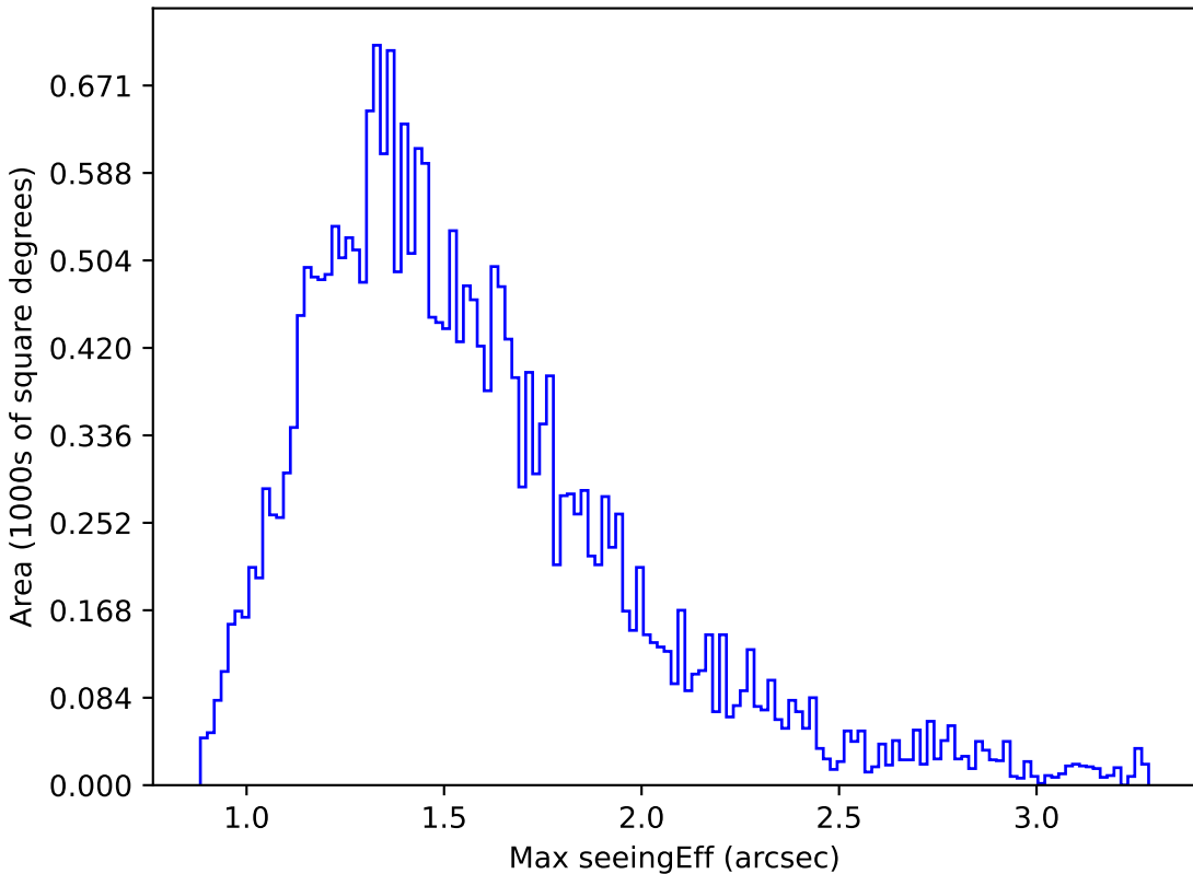
noroll_v3.4_10yrs Yr 1 i band: Max seeingEff
