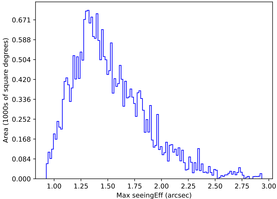
noroll_v3.4_10yrs Yr 1 g band: Max seeingEff
