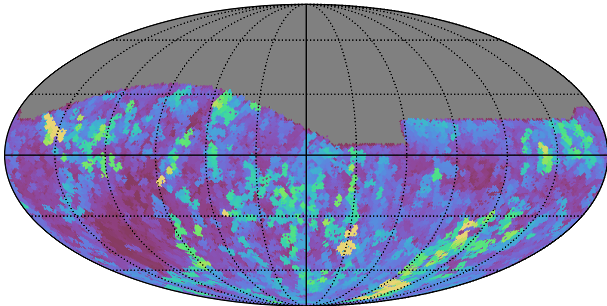
noroll_v3.4_10yrs Yr 1 all bands: Max seeingEff
