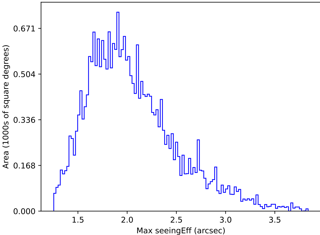
noroll_v3.4_10yrs Yr 1 all bands: Max seeingEff
