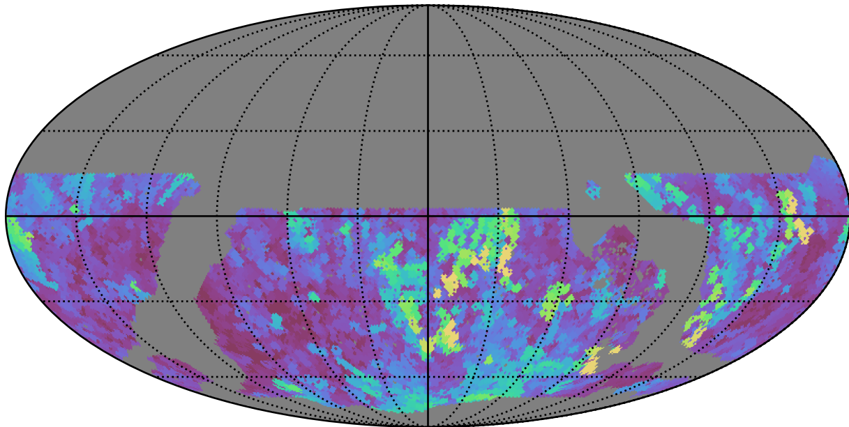
noroll_v3.4_10yrs WFD z band: Max seeingEff
