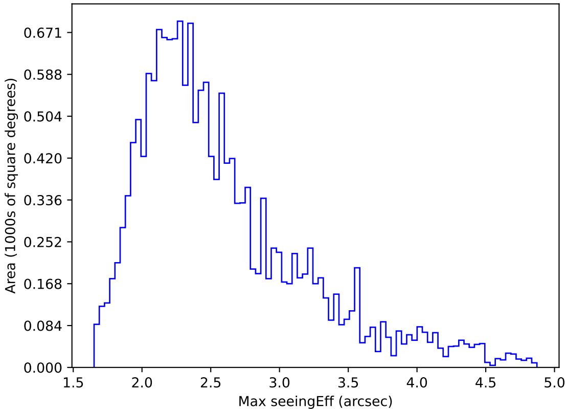
noroll_v3.4_10yrs WFD z band: Max seeingEff
