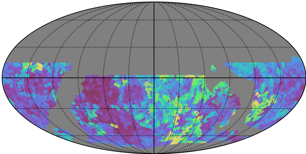
noroll_v3.4_10yrs WFD u band: Max seeingEff
