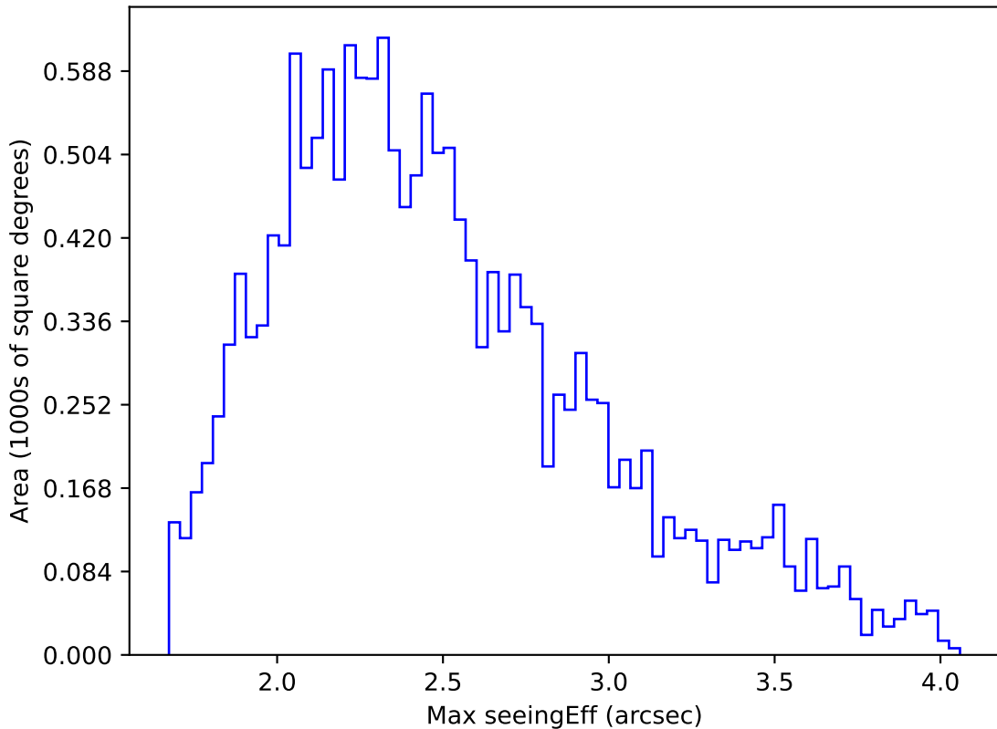
noroll_v3.4_10yrs WFD u band: Max seeingEff
