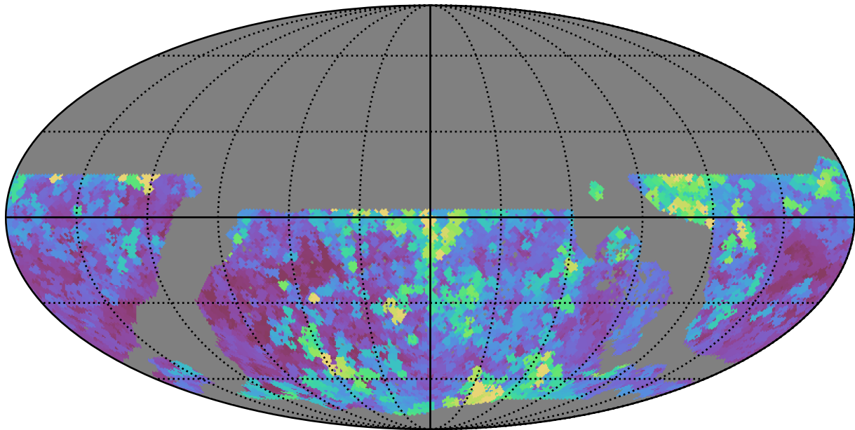
noroll_v3.4_10yrs WFD r band: Max seeingEff
