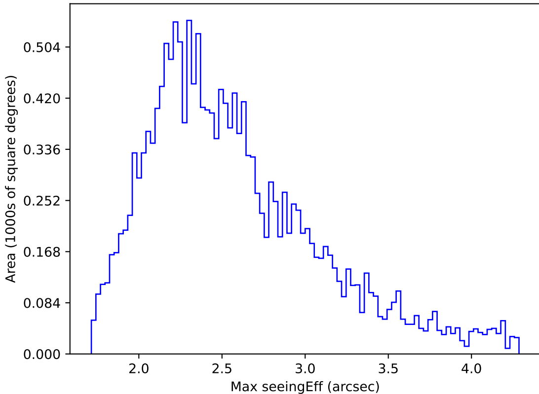
noroll_v3.4_10yrs WFD r band: Max seeingEff
