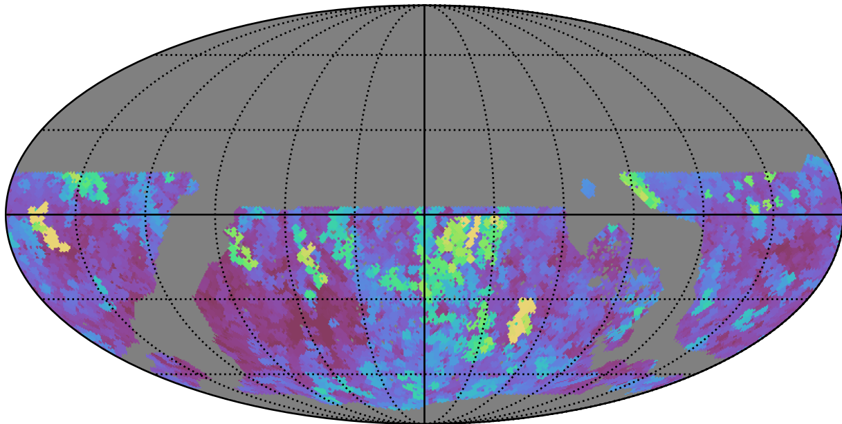
noroll_v3.4_10yrs WFD i band: Max seeingEff
