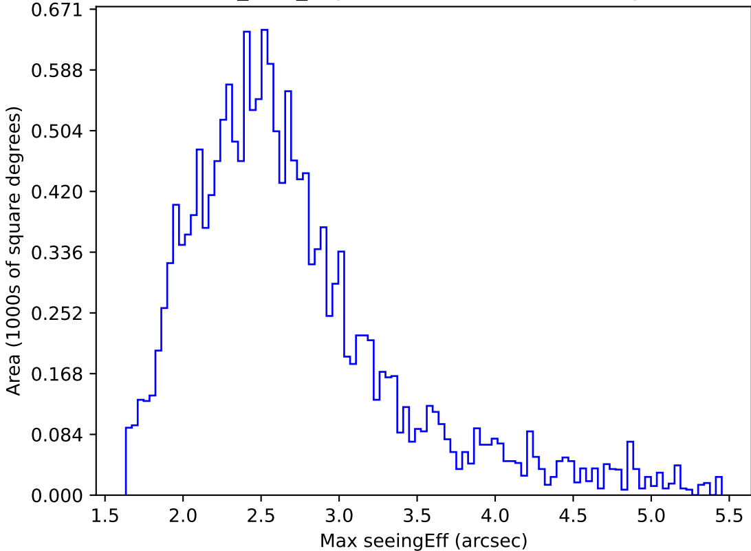
noroll_v3.4_10yrs WFD i band: Max seeingEff
