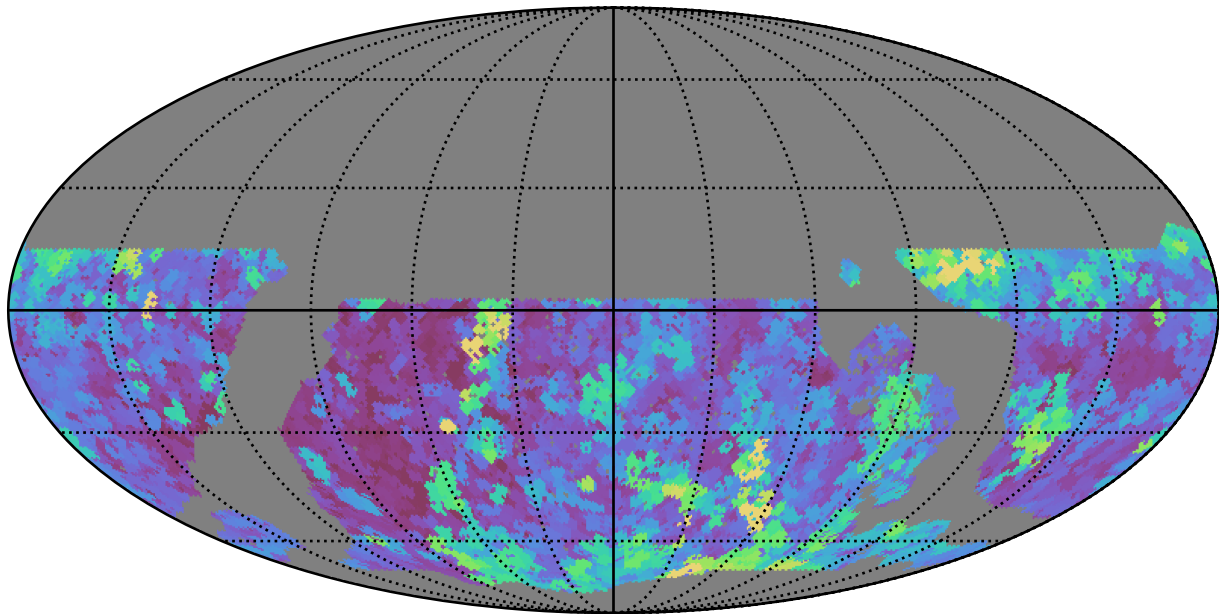
noroll_v3.4_10yrs WFD g band: Max seeingEff
