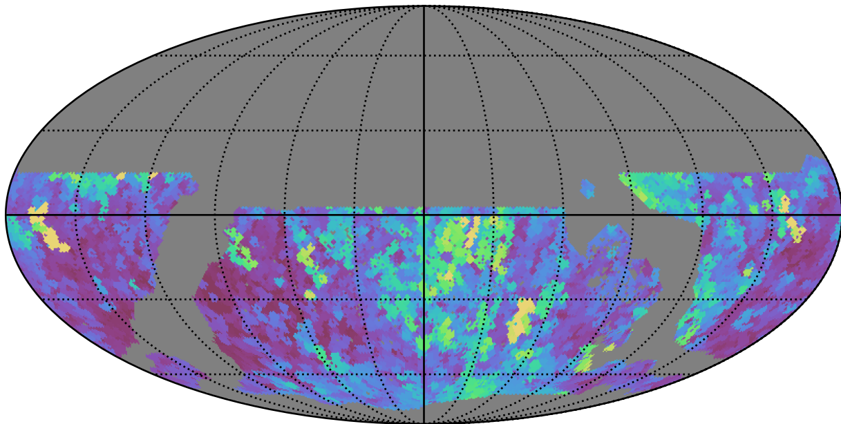
noroll_v3.4_10yrs WFD all bands: Max seeingEff
