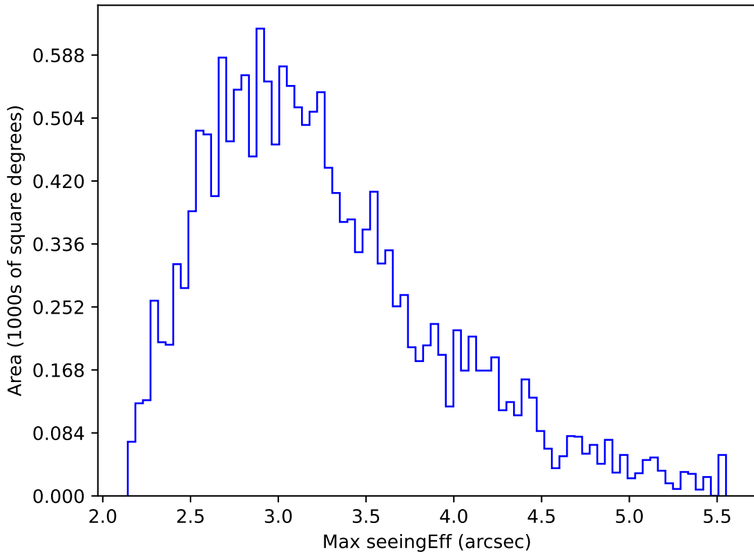
noroll_v3.4_10yrs WFD all bands: Max seeingEff
