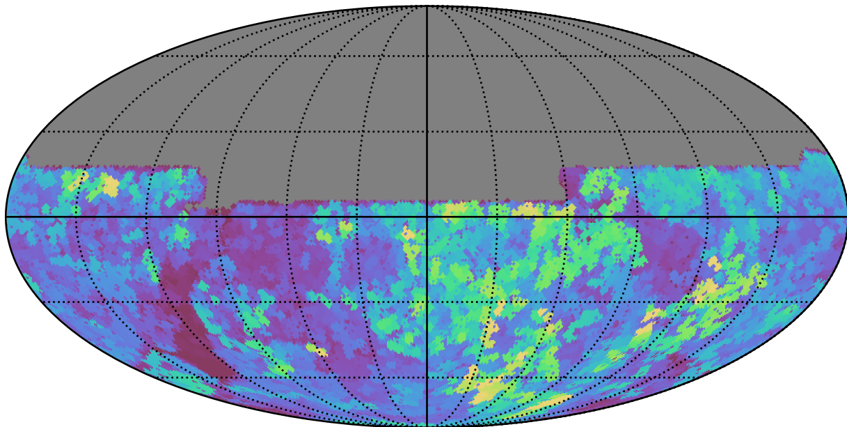
noroll_v3.4_10yrs All sky u band: Max seeingEff
