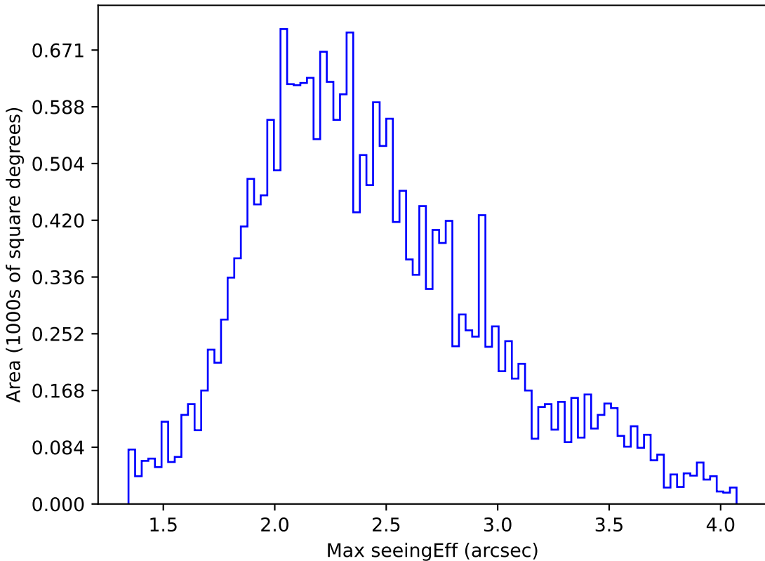
noroll_v3.4_10yrs All sky u band: Max seeingEff
