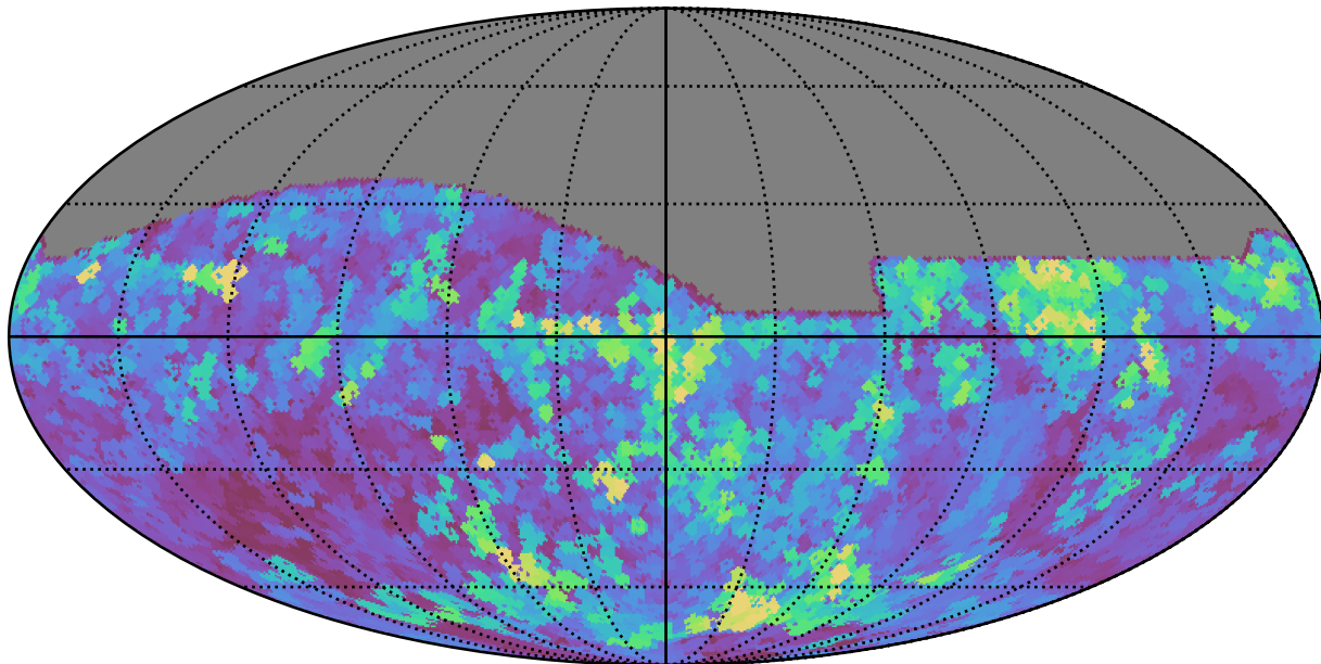
noroll_v3.4_10yrs All sky r band: Max seeingEff
